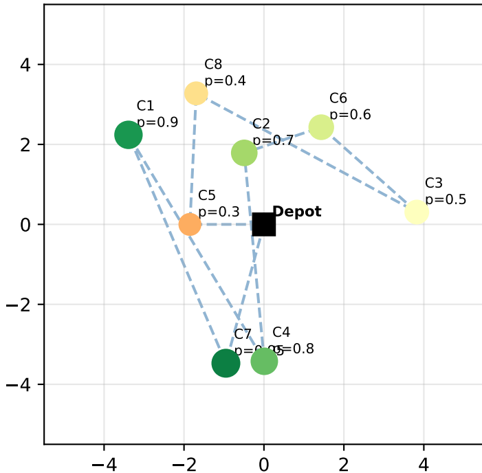
A Priori Route (all customers planned) Node size \propto presence probability
