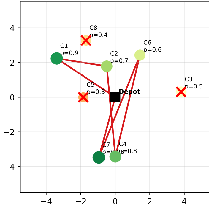
Realized Route (low-prob customers absent) Cross = customer not present
