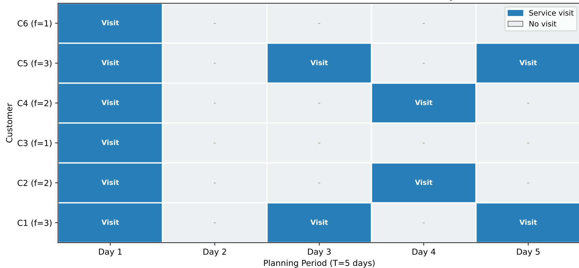
Periodic VRP (PVRP): Visit Schedule over T=5 Days
