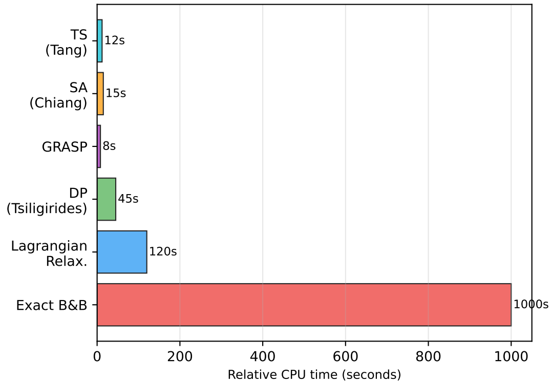
OP Algorithm Speed (lower = faster)
