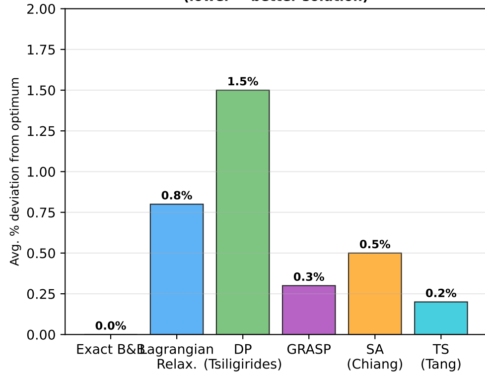
OP Algorithm Quality (lower = better solution)
