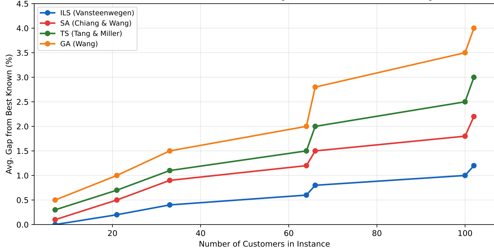
TOP Heuristic Comparison on Chao-Golden-Wasil Benchmark (ILS = Iterated Local Search; SA = Simulated Annealing; TS = Tabu Search; GA = Genetic Algorithm)
