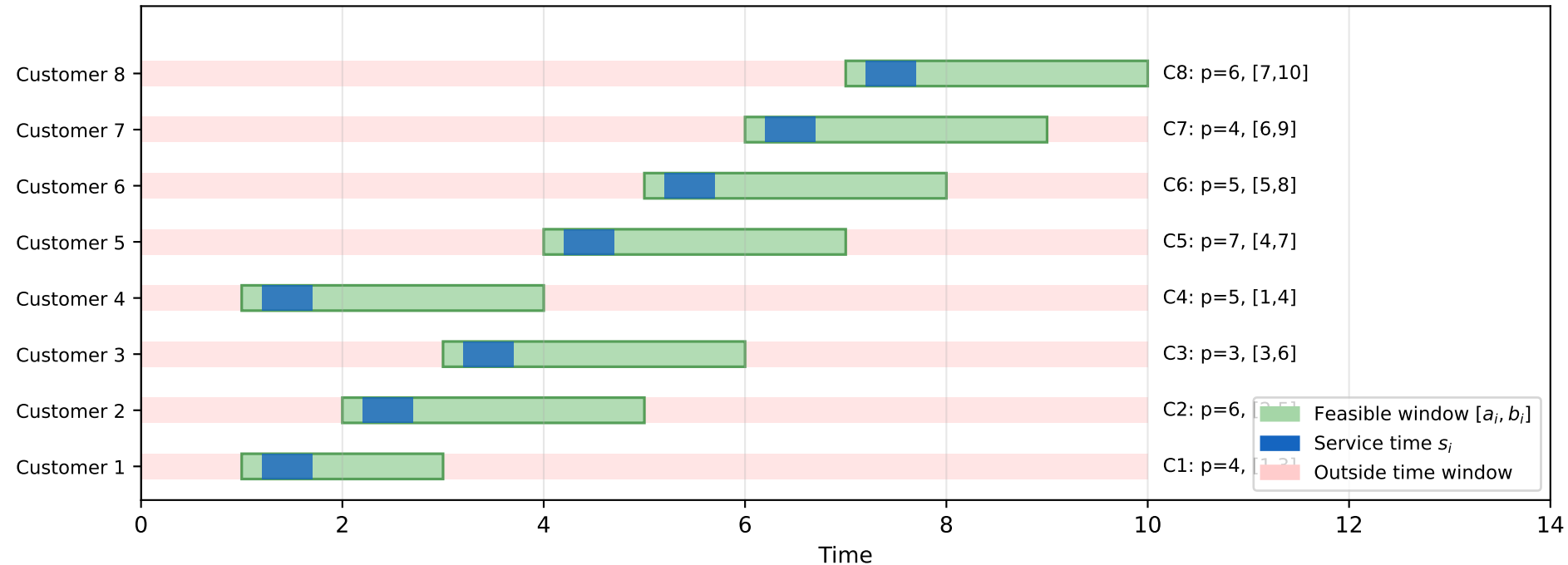
Time-Window Constraints in TW-OP / TW-TOP Vehicle must arrive in [a_i, b_i] for customer i
