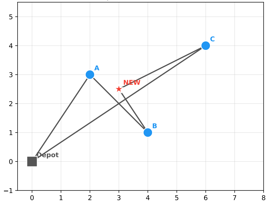
After: cheapest insertion between B and C
