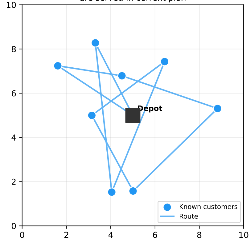
Reactive: only known requests are served in current plan
