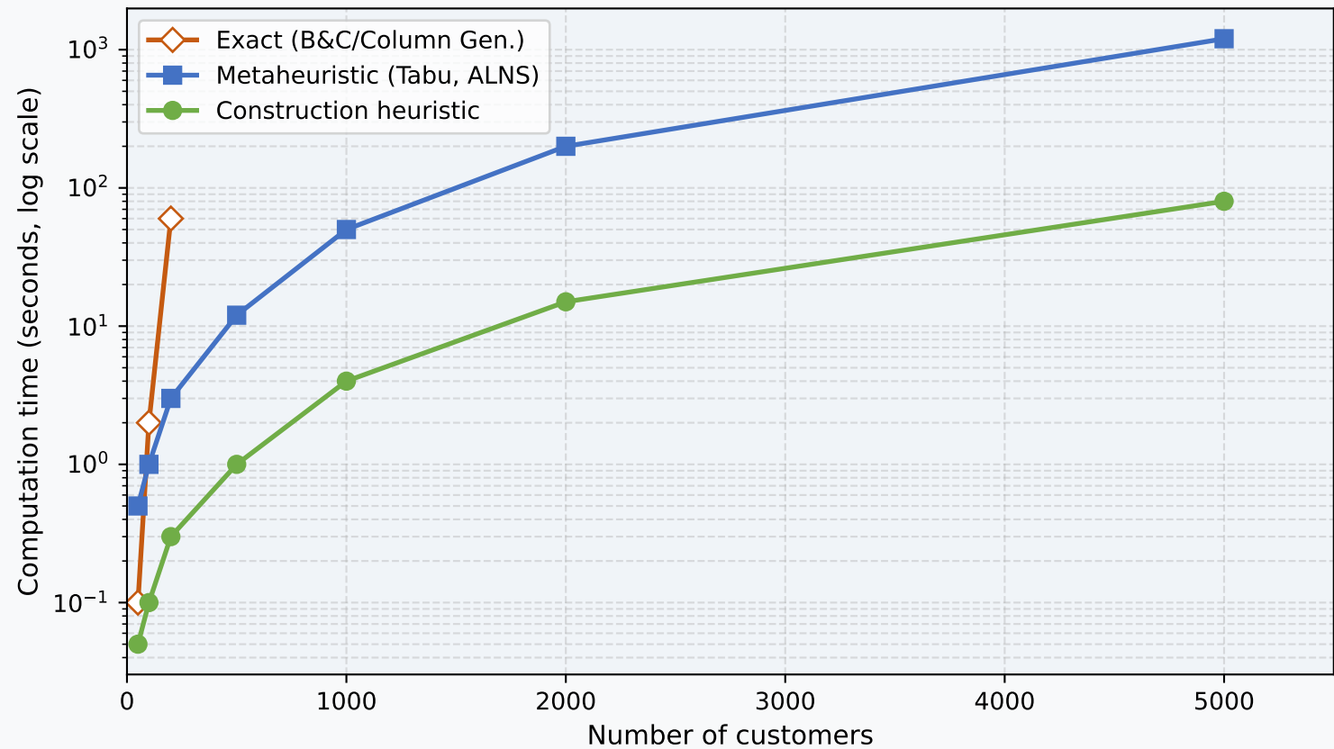
Schematic Performance vs. Problem Size for Different Algorithm Classes
