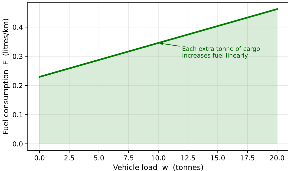
Fuel Consumption vs. Payload (linear in load — heavier = more fuel)
