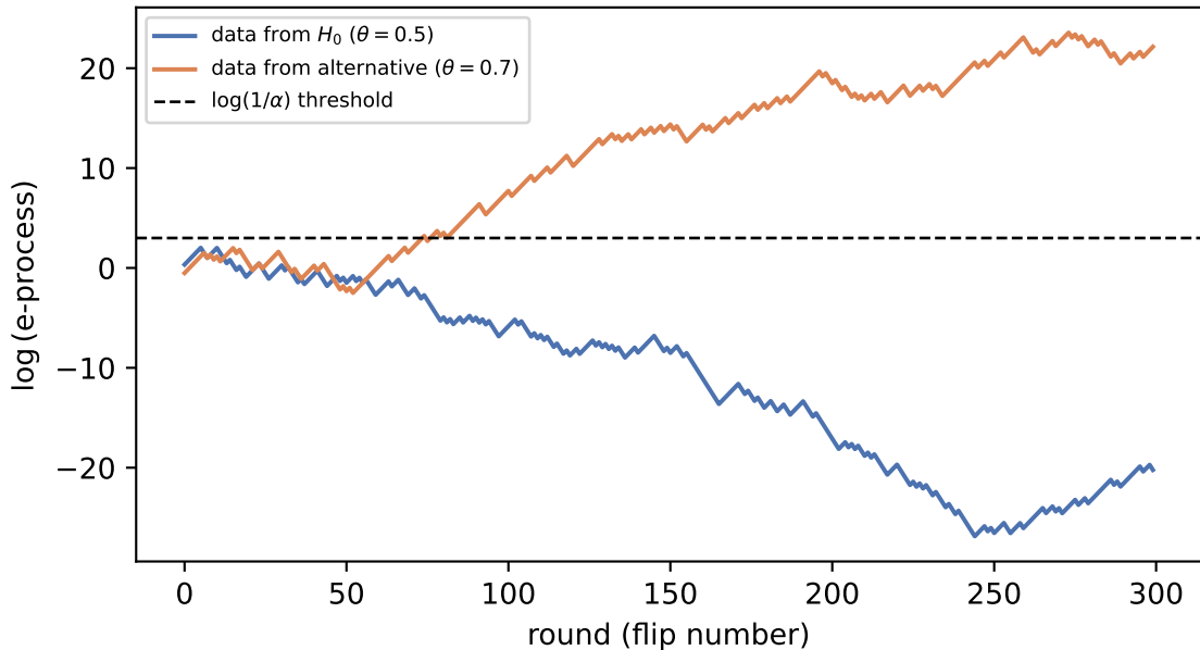
Growth of the likelihood-ratio e-process M_n
