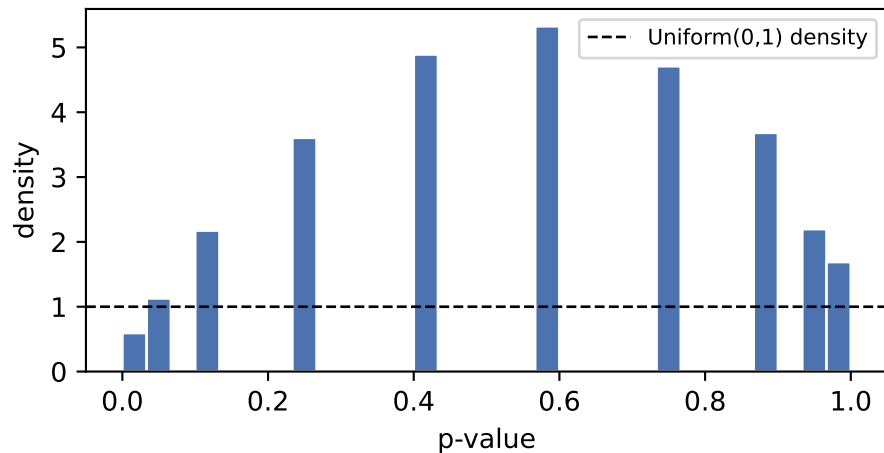
P-values under H_0 (stochastically \geq Uniform(0,1))
