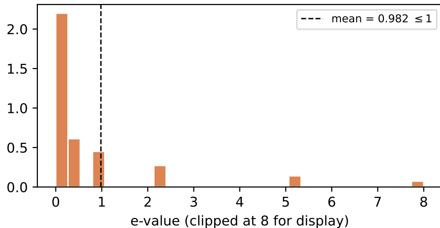
E-values under H_0 (right-skewed, mean \leq 1 )
