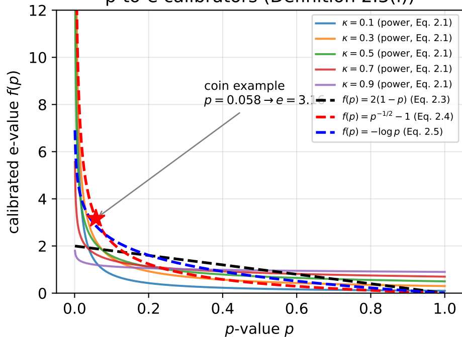
p-to-e calibrators (Definition 2.3(i))
