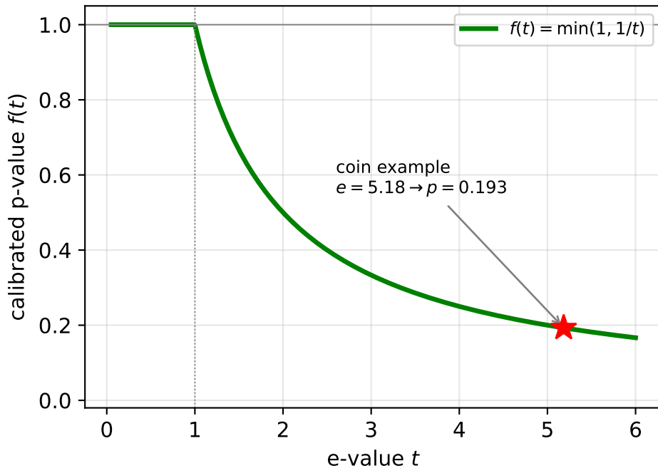
The unique admissible e-to-p calibrator (Proposition 2.4, from Markov's inequality)
