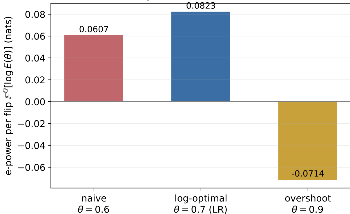
Coin example: H_0: \theta = 0.5 vs. true \theta = 0.7
