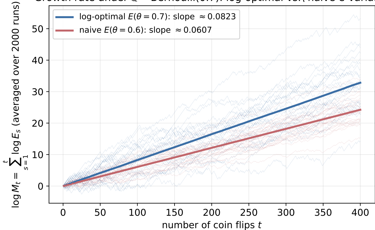
Growth rate under \mathcal{Q} = \text{Bernoulli}(0.7) : log-optimal vs. naive e-variable
