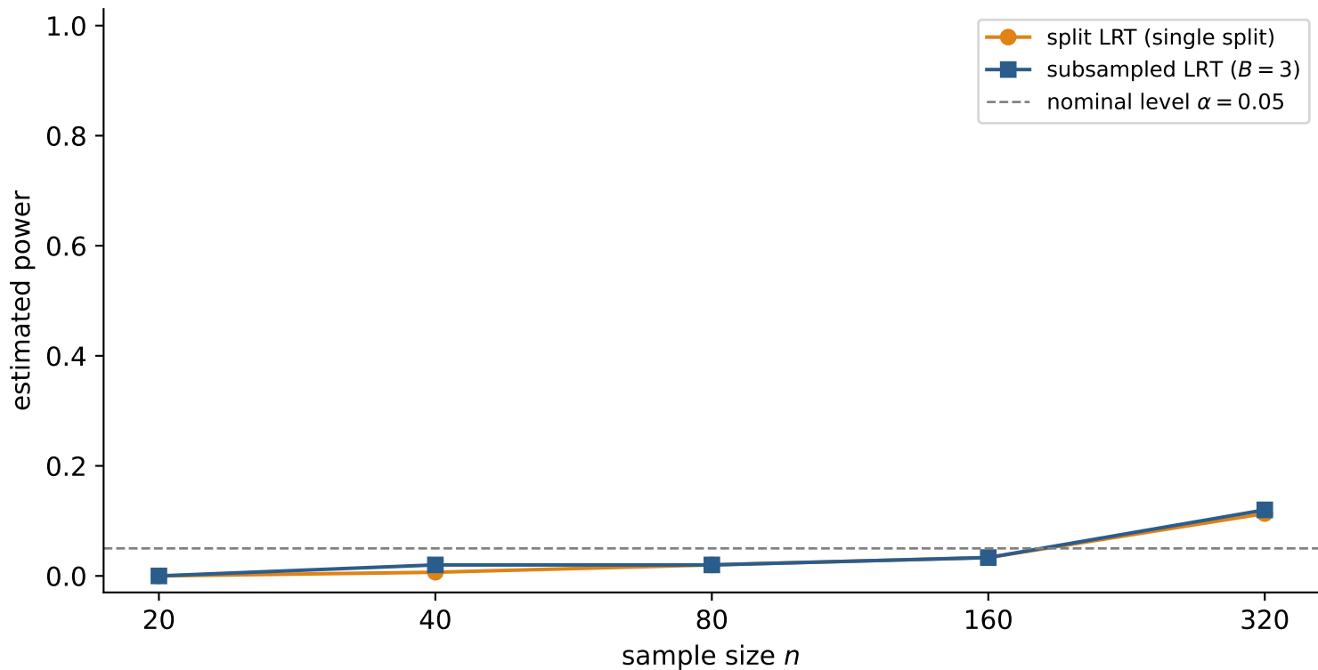
Power of the split/subsampled LR e-value test H_0 : \mu_1 = \mu_2 vs. mixture with true gap \mu_1 - \mu_2 = -2 \times 0.55
