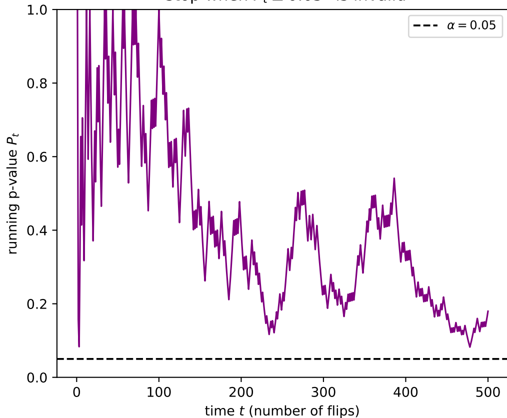
P-value process under H_0 : "stop when P_t \leq 0.05 " is invalid
