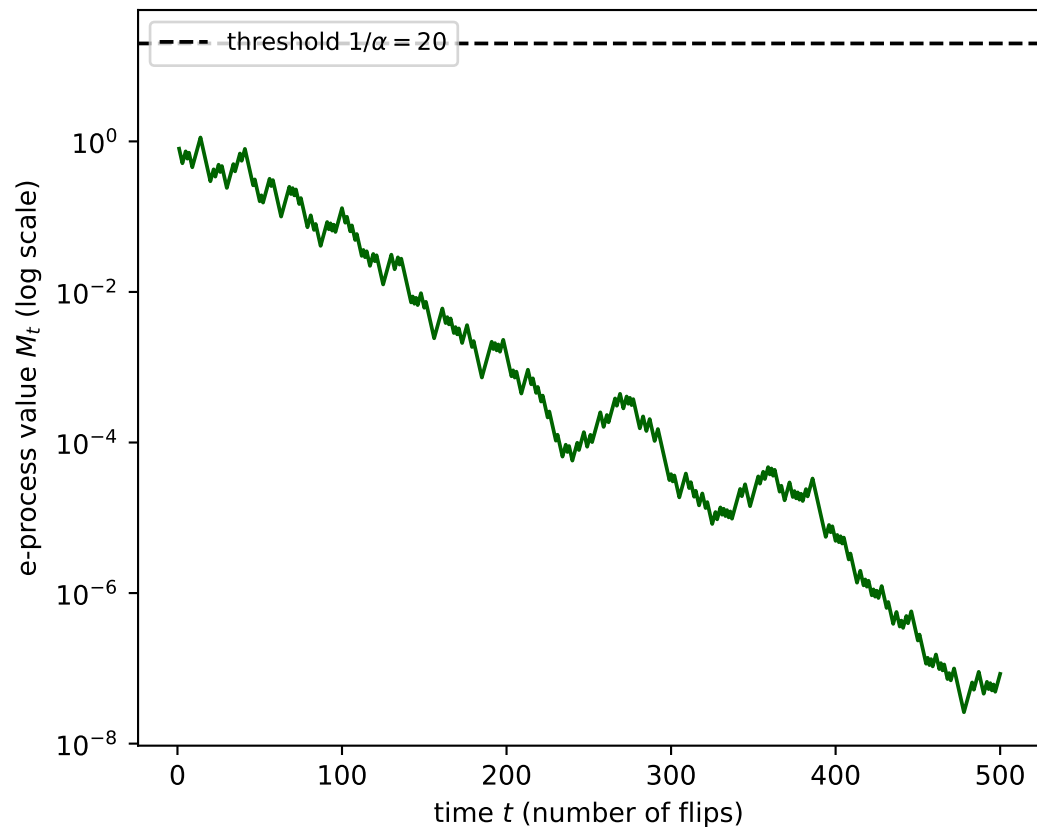
Same null data, e-process: stopping any time keeps \mathbb{P}(M_t \geq 1/\alpha) \leq \alpha
