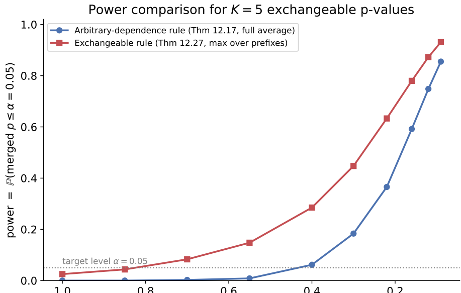
Figure: power gain from exploiting exchangeability
