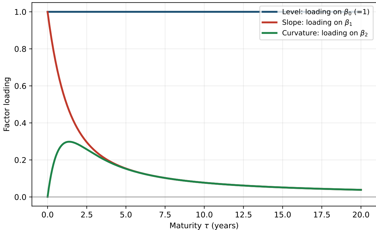
Nelson--Siegel factor loadings ( \lambda = 1.3 )
