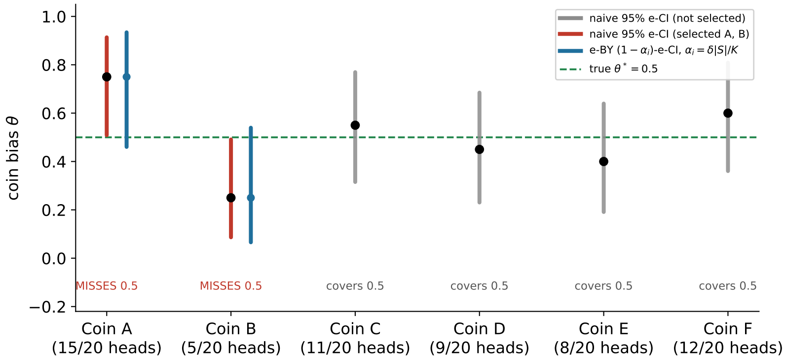
Naive 95% e-CIs (gray/red) vs. e-BY-corrected 98.33% e-CIs (blue) for the two selected 'most extreme' coins A, B
