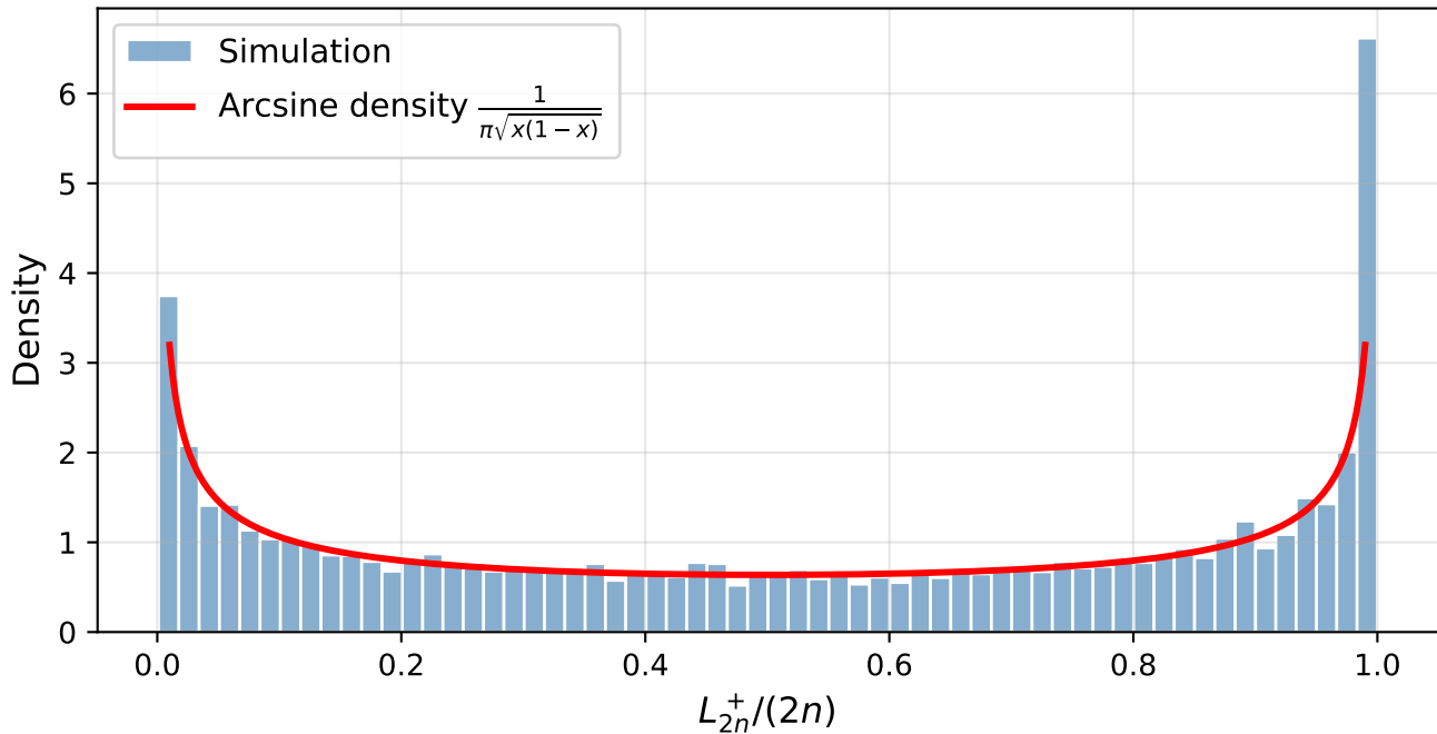
Arcsine Law: simulation vs theory ( n = 500 , R = 10,000 )
