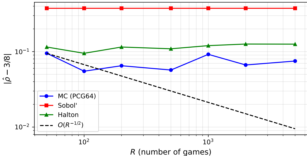
2-D game: MC vs QMC convergence to \rho(2, 3) = 3/8
