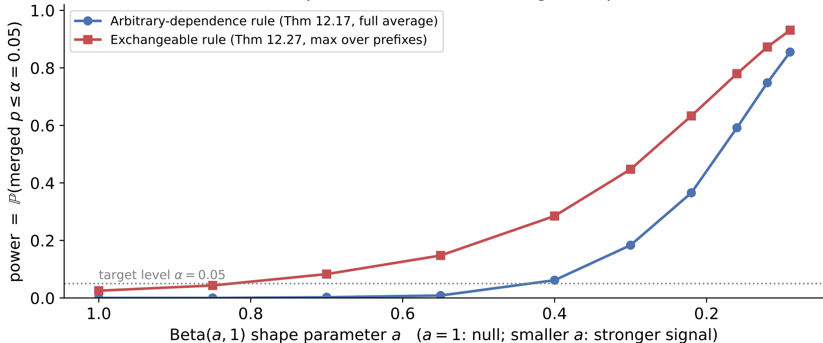
Power comparison for K = 5 exchangeable p-values
