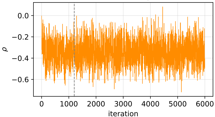
MALA trace: \rho
