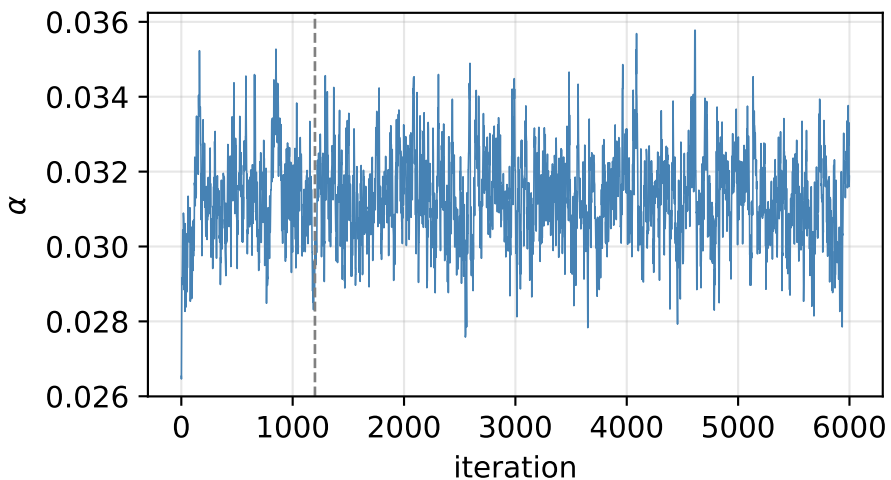
MALA trace: \alpha
