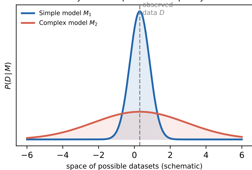
Why evidence penalizes complexity
