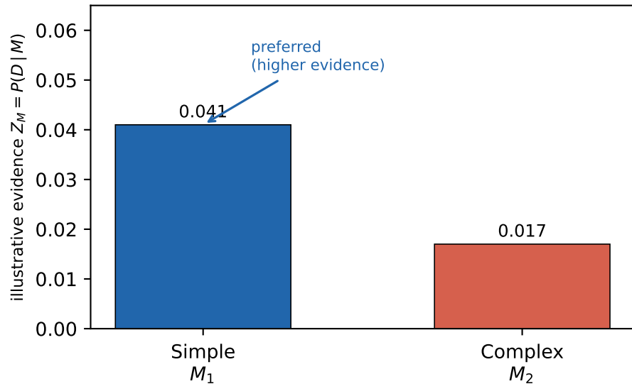
Toy evidence comparison
