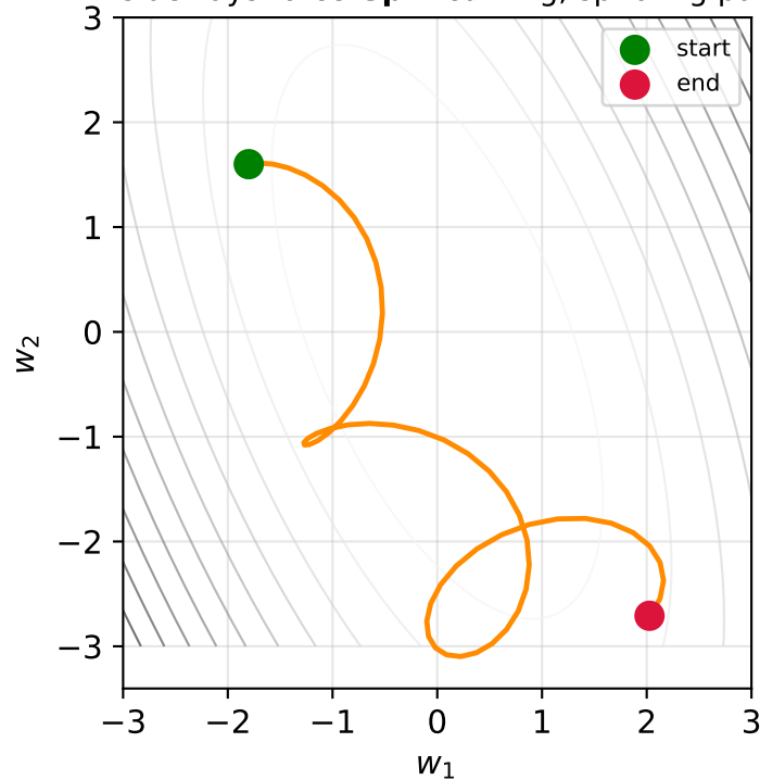
Magnetic HMC: + sideways force \mathbf{Gp} -- curving, spiraling path
