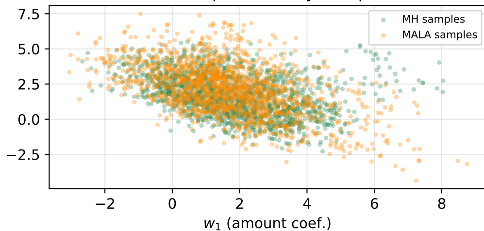
Posterior samples (2D toy sub-posterior)
