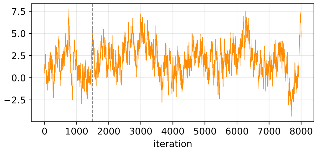
MALA trace: w_2 (budget-variance coef.)
