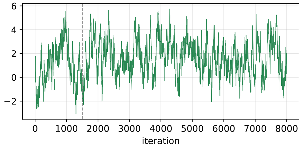
MH trace: w_2 (budget-variance coef.)
