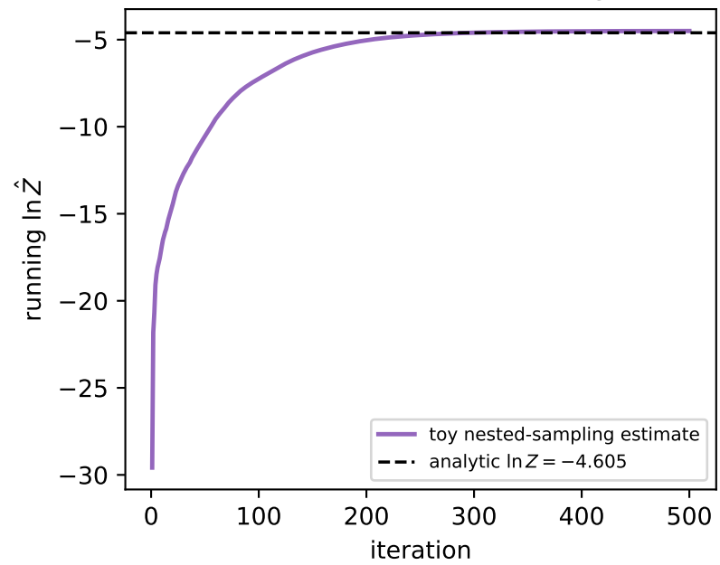
(c) Evidence estimate converges
