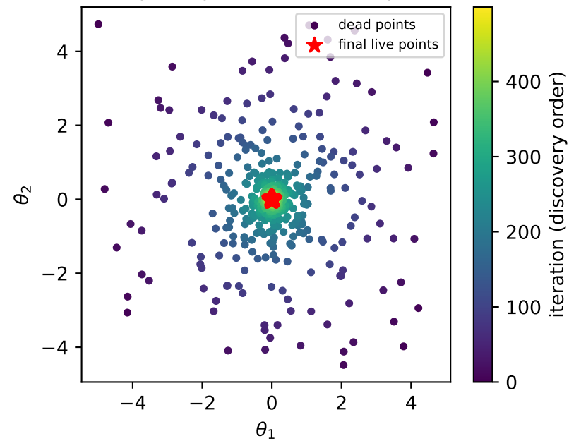
(a) Toy sampler: dead \& live points
