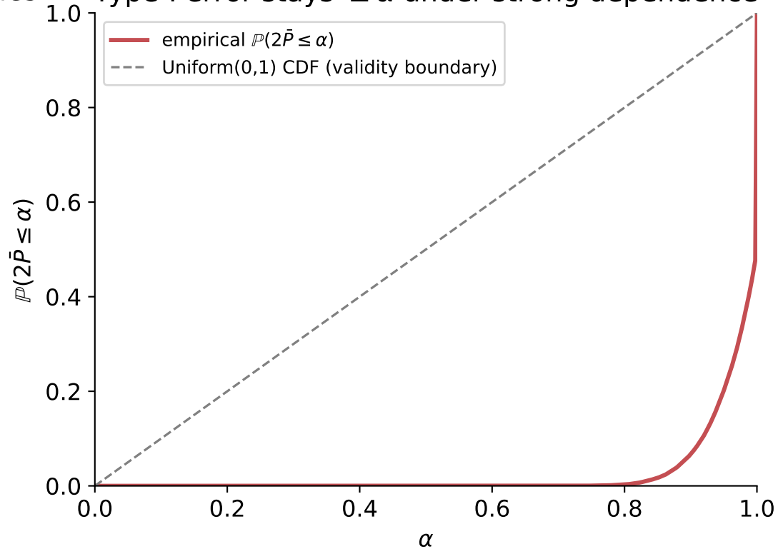
Type-I error stays \leq \alpha under strong dependence
