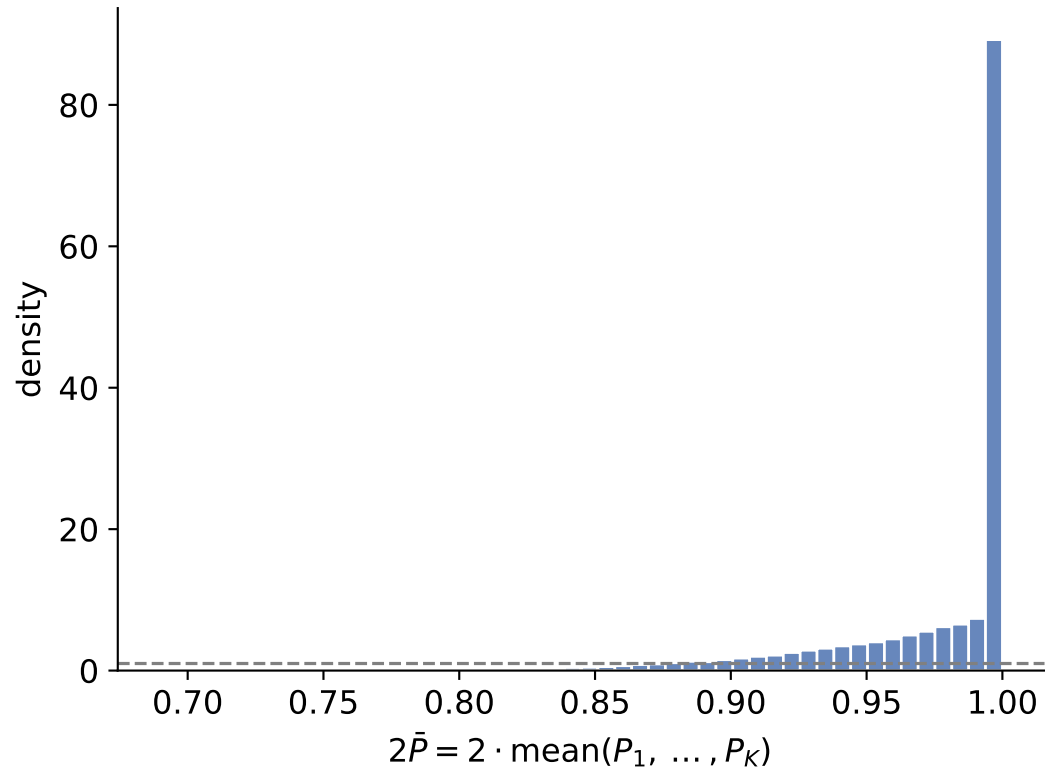
Histogram of 2\bar{P} , K = 8 strongly anti-dependent p-values
