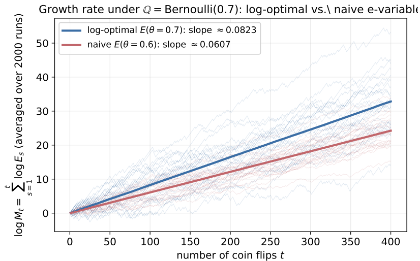
Figure: growth rate over repeated coin flips
