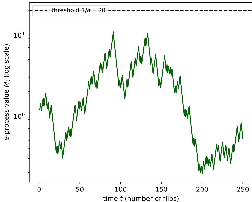
Same null data, e-process: stopping any time keeps \mathbb{P}(M_t \geq 1/\alpha) \leq \alpha
