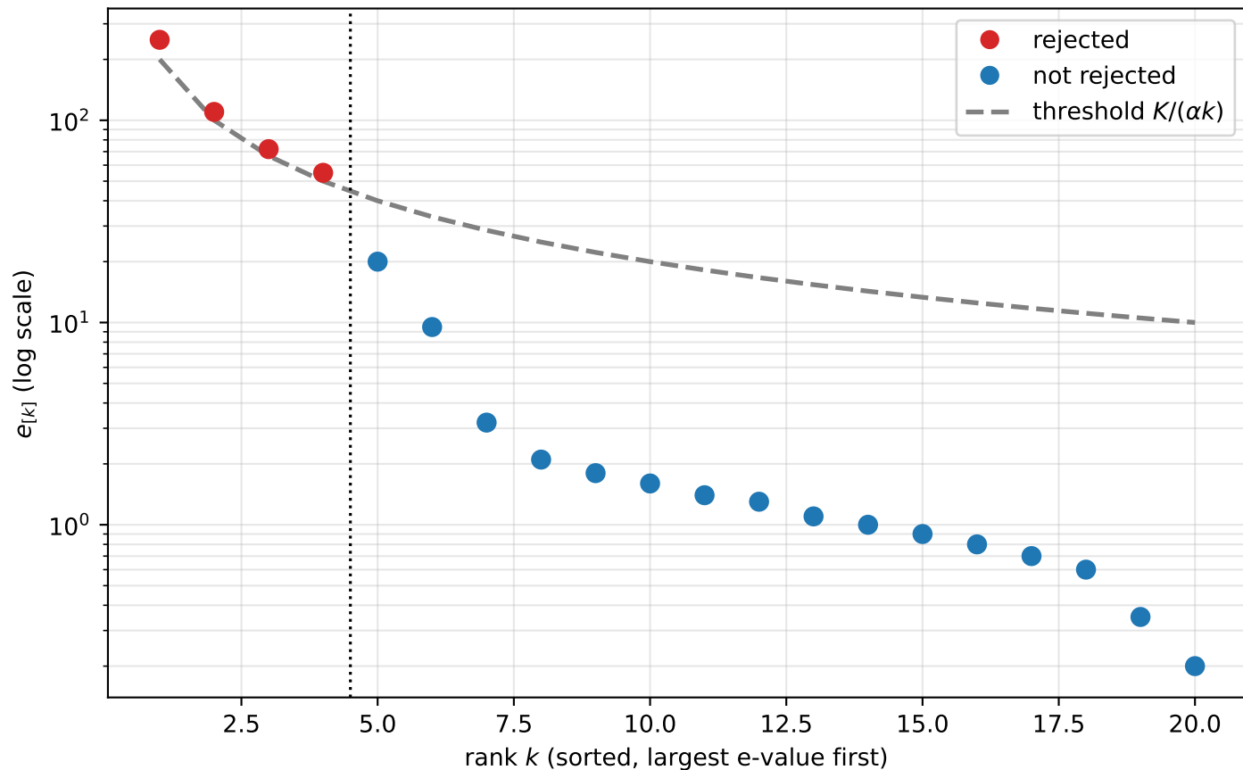
e-BH procedure on 20 e-values ( K = 20 , \alpha = 0.1 ): k^* = 4 rejections
