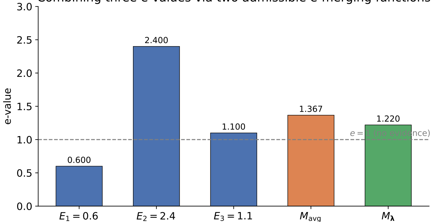
Combining three e-values via two admissible e-merging functions
