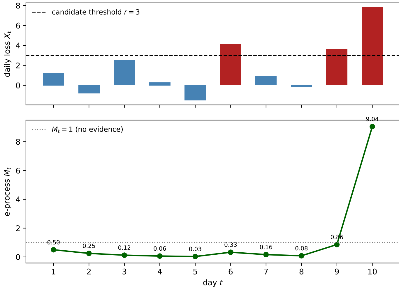
Backtesting H_0 : \text{VaR}_{0.95}(F) \leq r with a monotone backtest e-statistic
