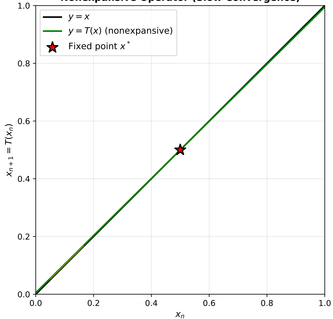
Nonexpansive Operator (Slow Convergence)
