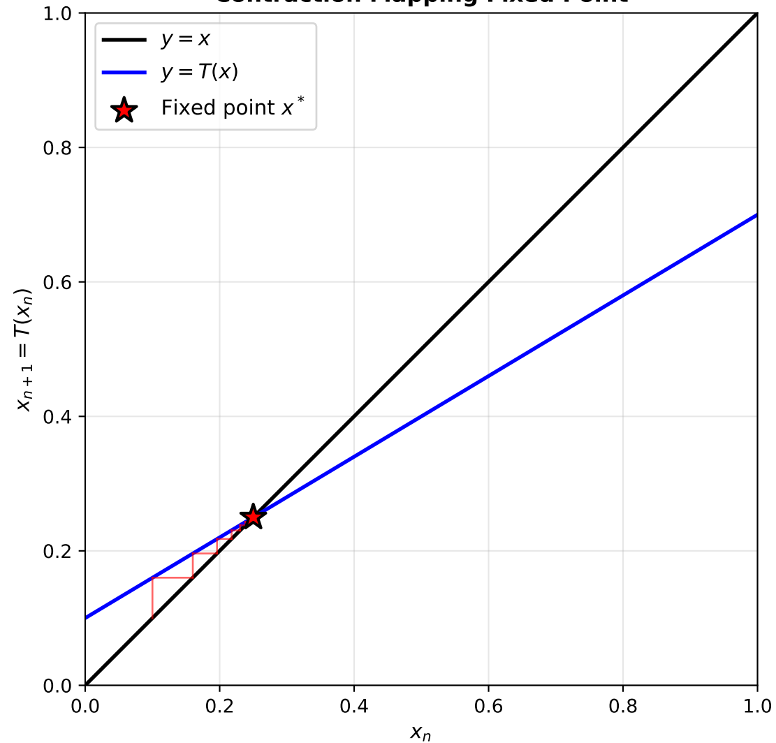
Contraction Mapping Fixed Point
