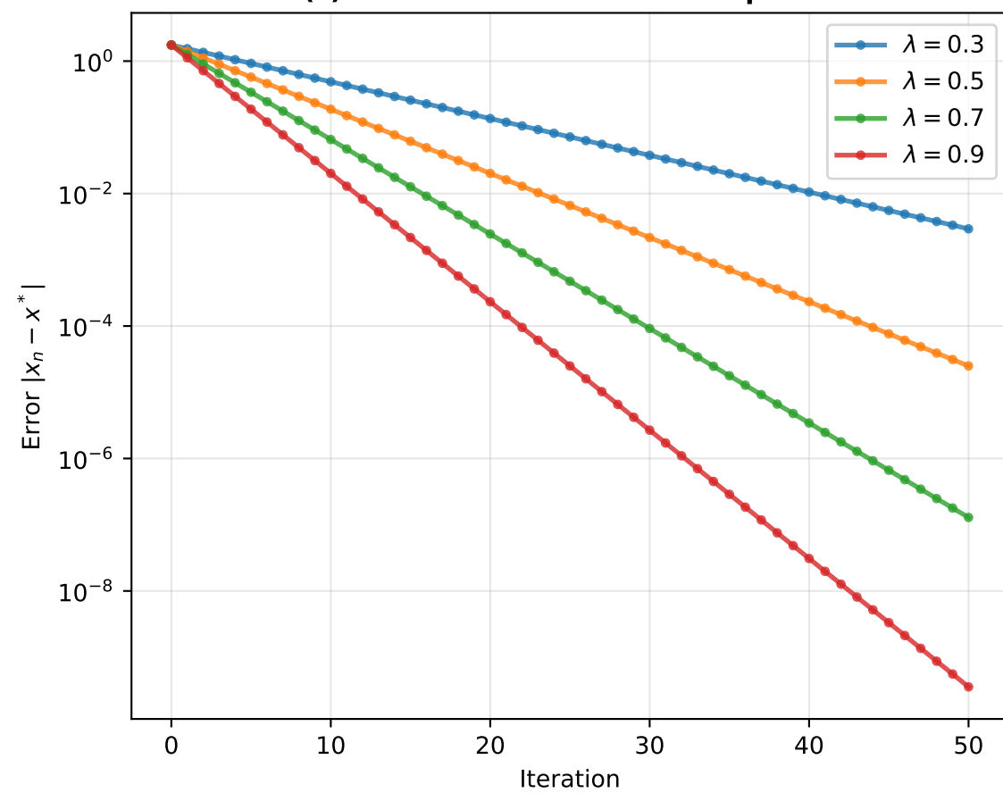
(c) KM Iteration: Different Stepsizes
