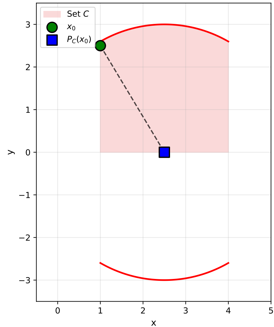
Projection onto Convex Set C
