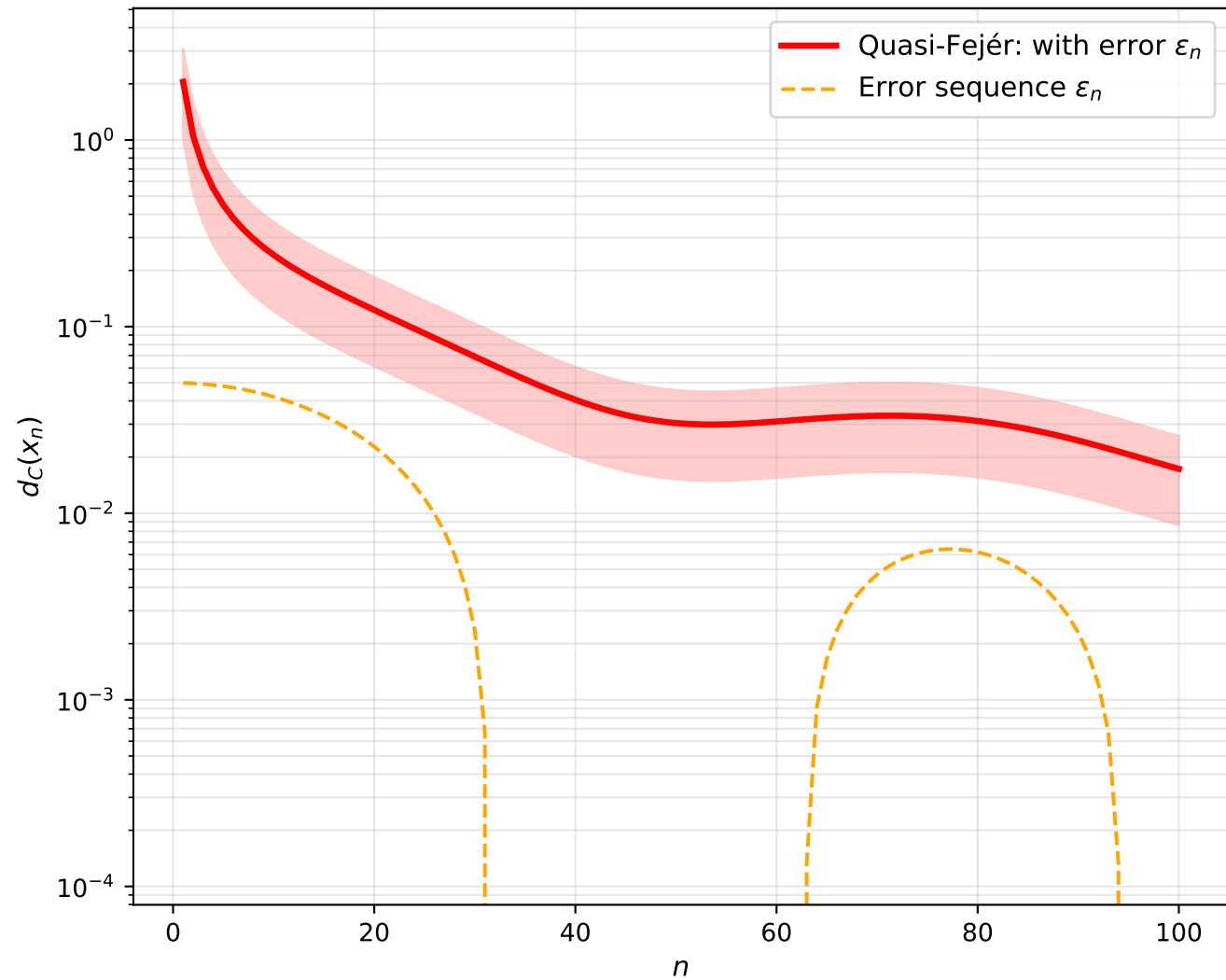
(b) Quasi-Fejér Monotonicity (with errors)
