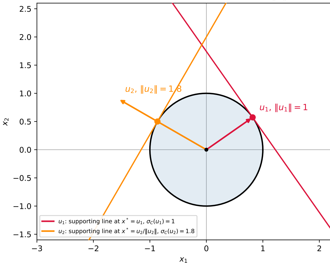
Support function of the unit disk: \sigma_C(u) = \|u\|
