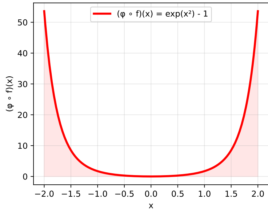
Result: Convex Composition
