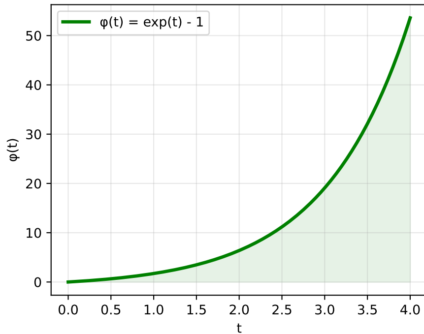
Step 2: Increasing Convex \varphi(t)
