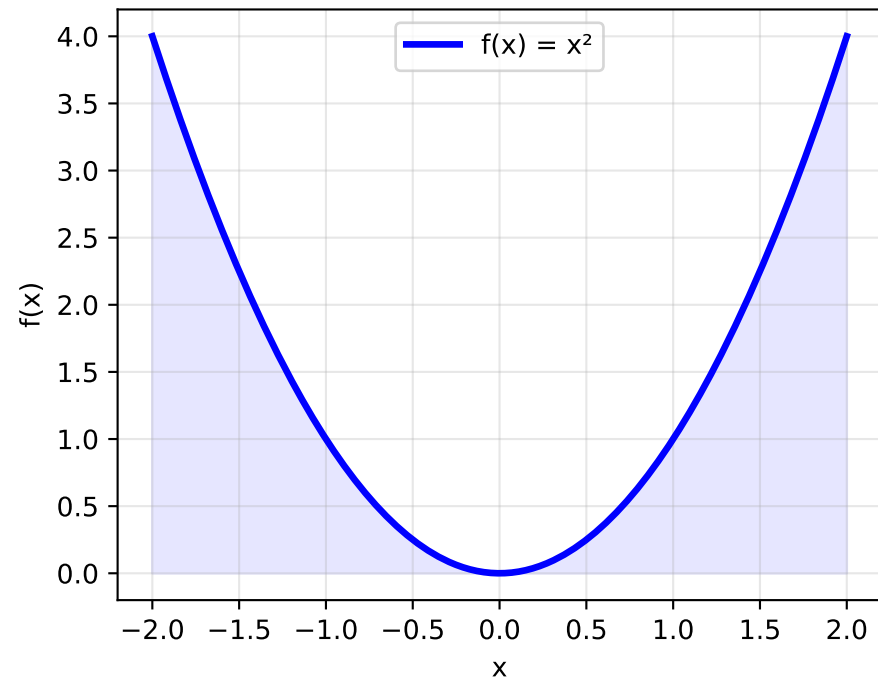
Step 1: Convex f(x)
