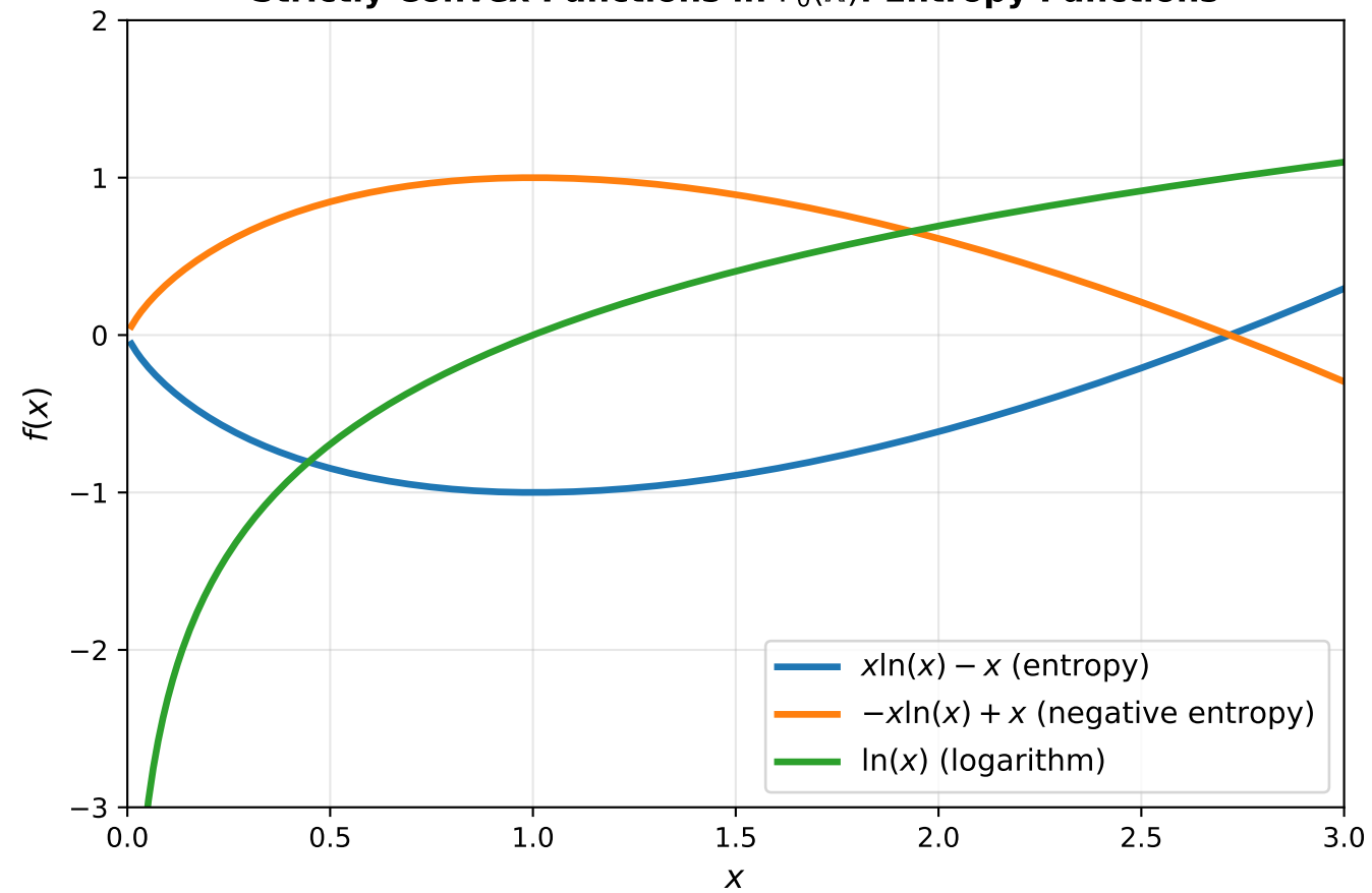
Strictly Convex Functions in \Gamma_0(\mathbb{R}) : Entropy Functions
