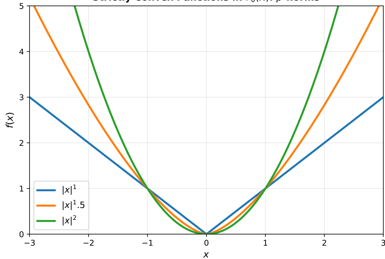
Strictly Convex Functions in \Gamma_0(\mathbb{R}) : p -norms
