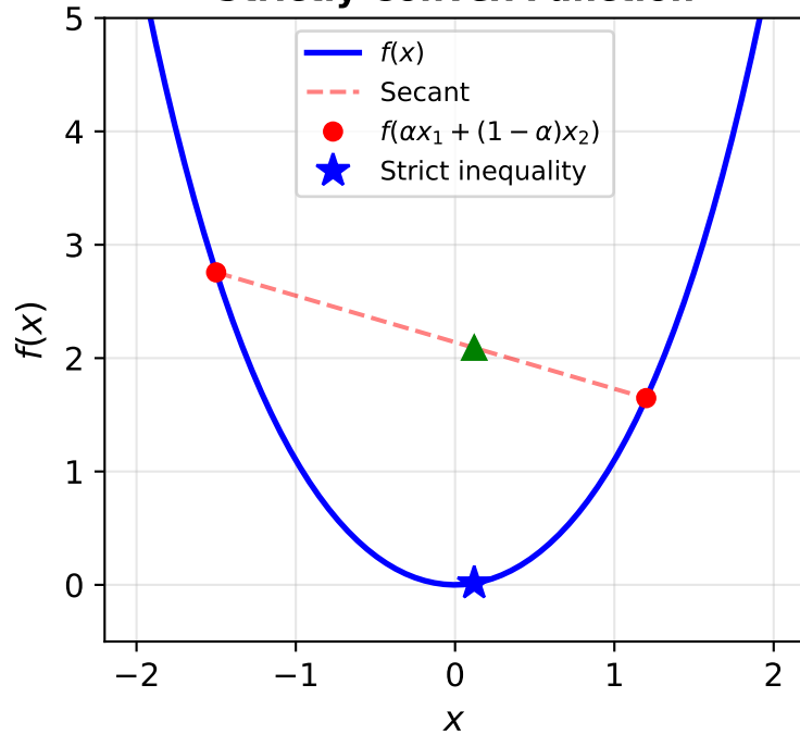
Strictly Convex Function
