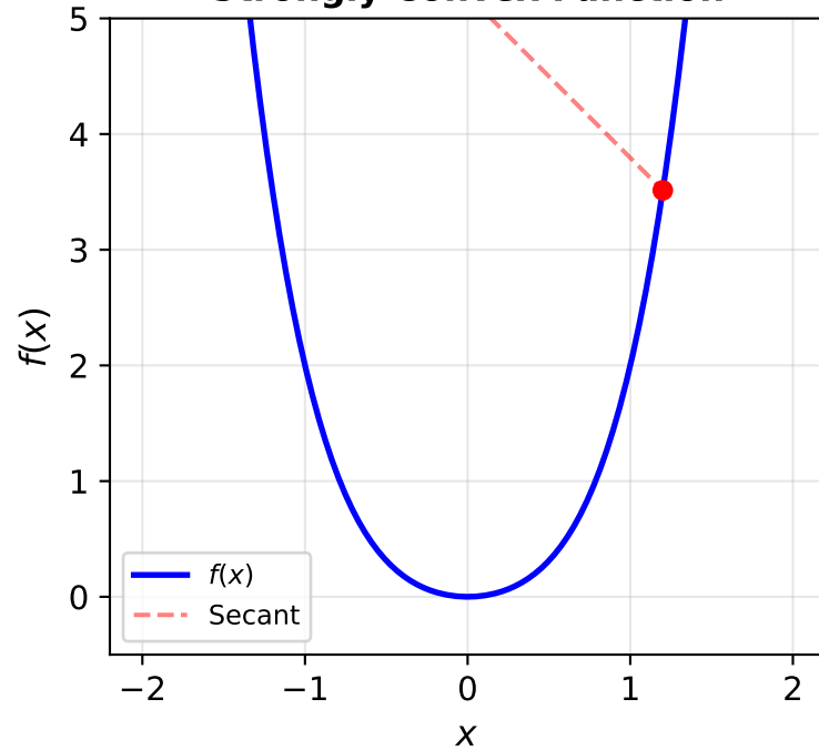
Strongly Convex Function
