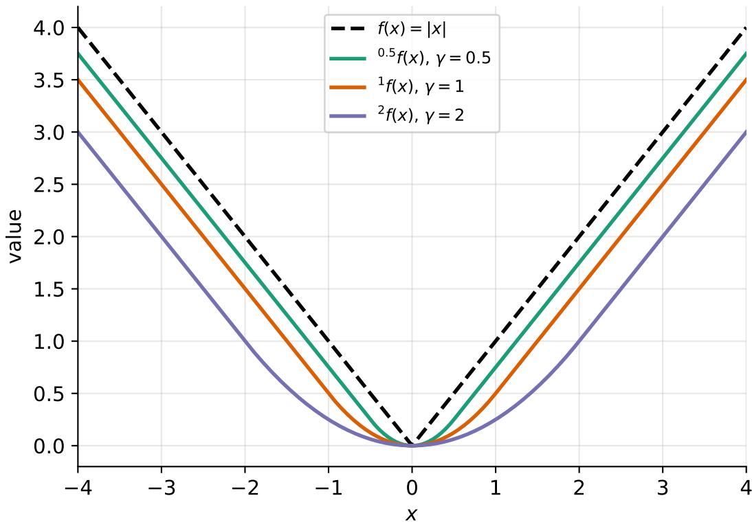
Moreau envelopes of f = |\cdot|
