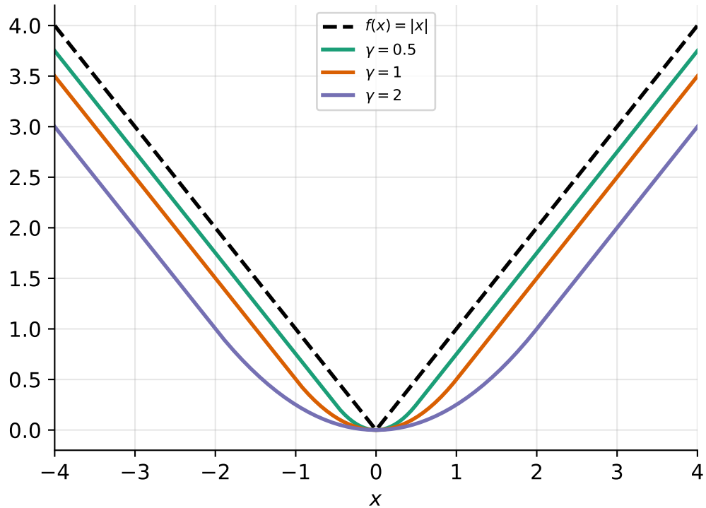
Moreau envelope \gamma f
