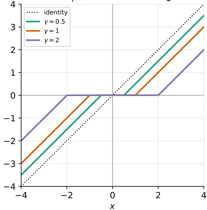
\text{Prox}_{\gamma f} (soft-thresholding)
