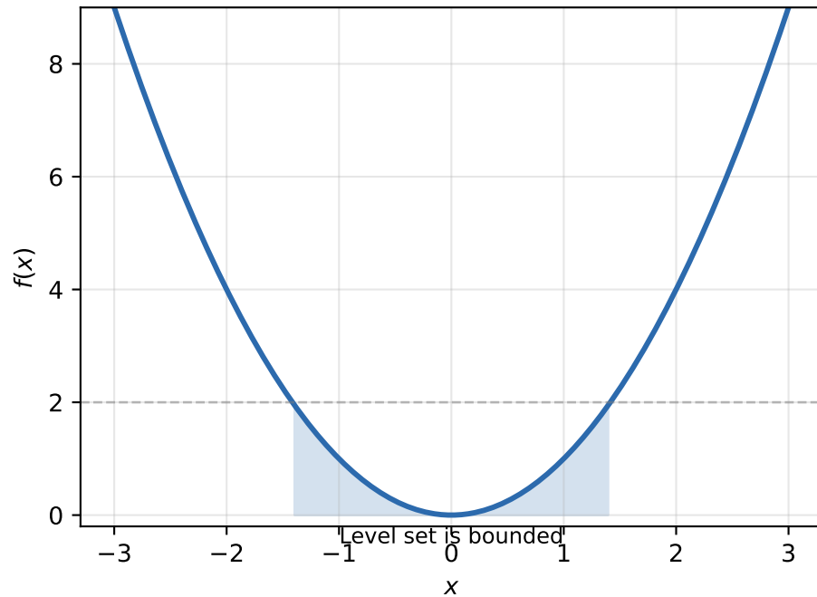
(b) Coercive: f(x) = x^2
