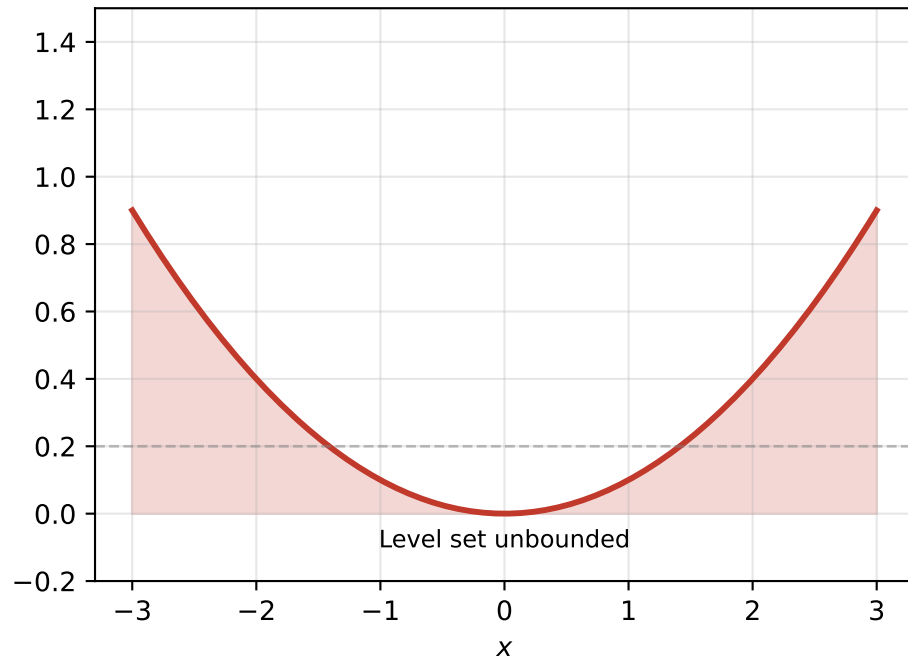
(a) Non-coercive: f(x) = 0.1x^2
