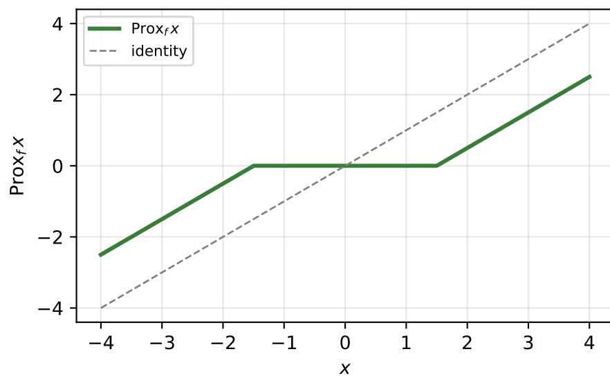
(c) \text{Prox}_f (soft thresholder)
