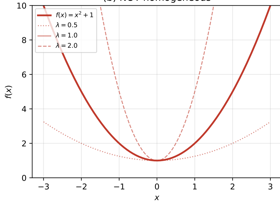
(b) NOT homogeneous
