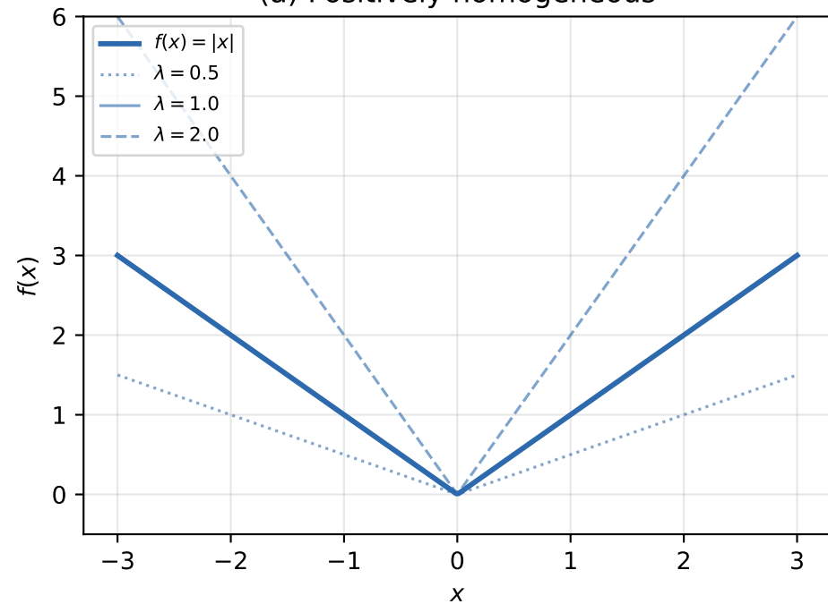
(a) Positively homogeneous
