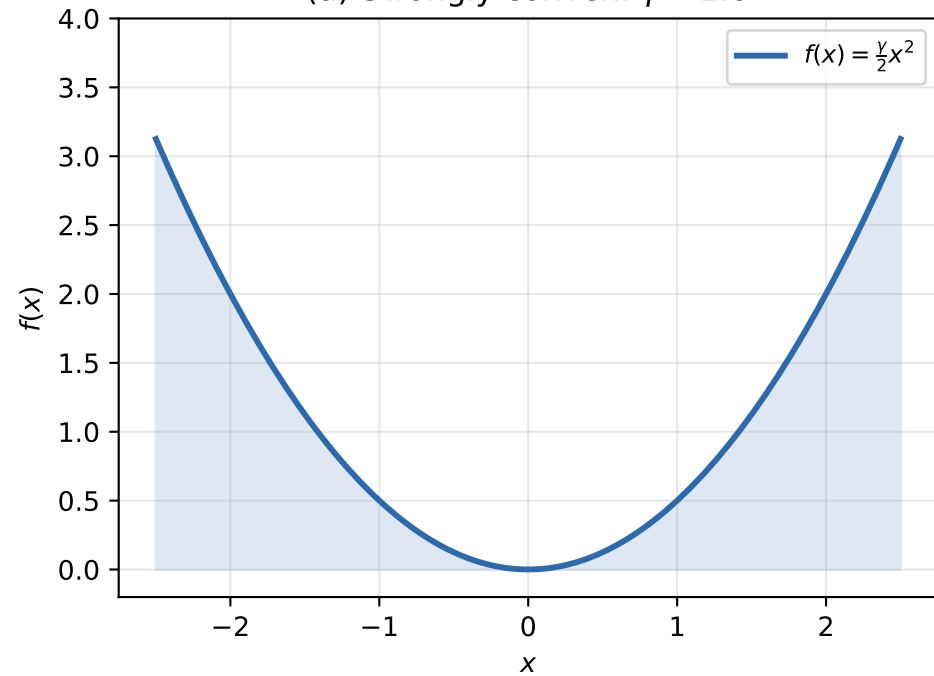
(a) Strongly convex: \gamma = 1.0
