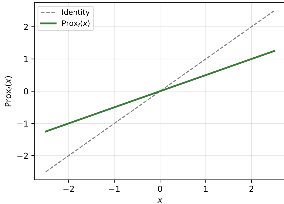
(b) Proximal operator
