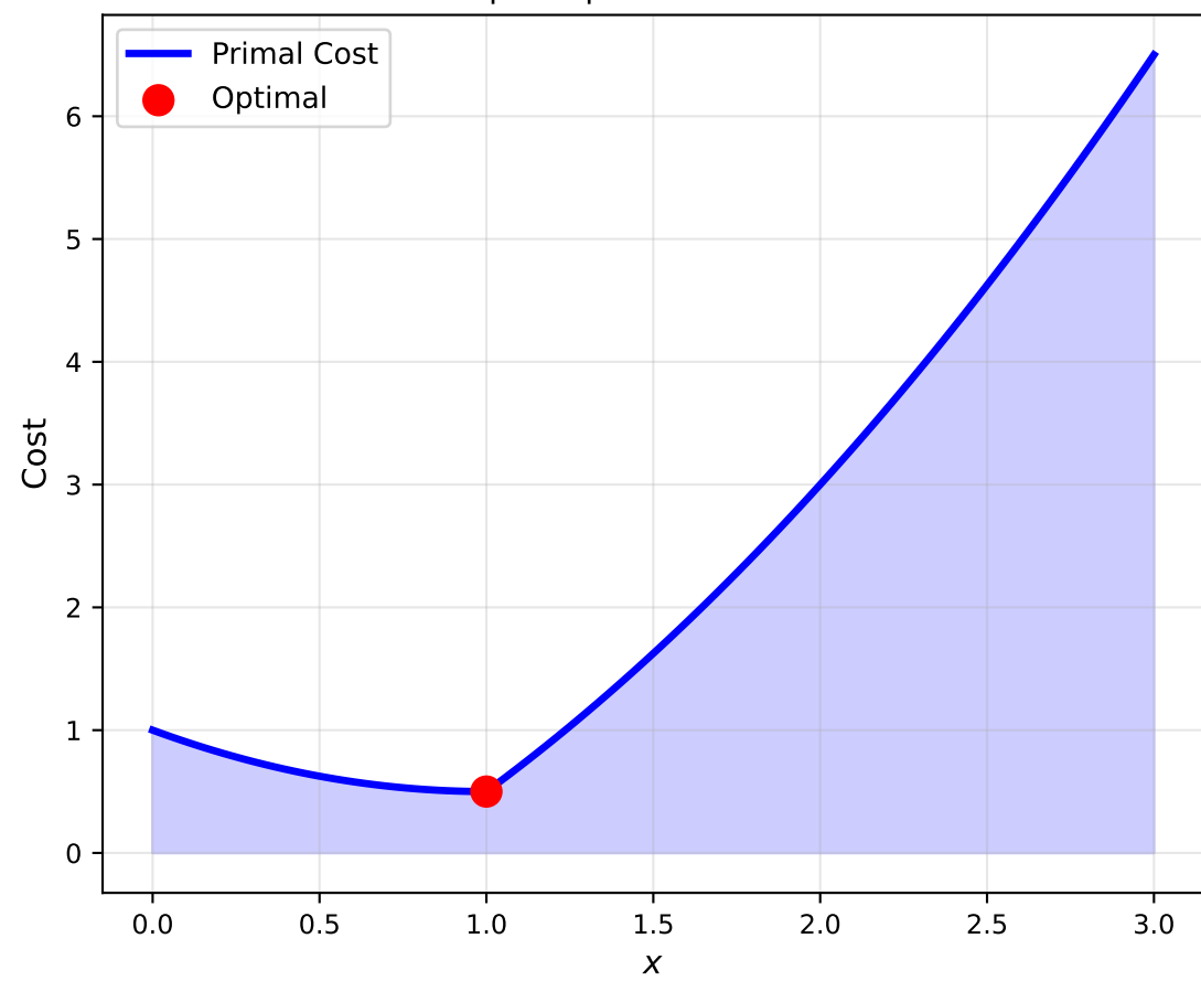
Example: Optimization Problem
