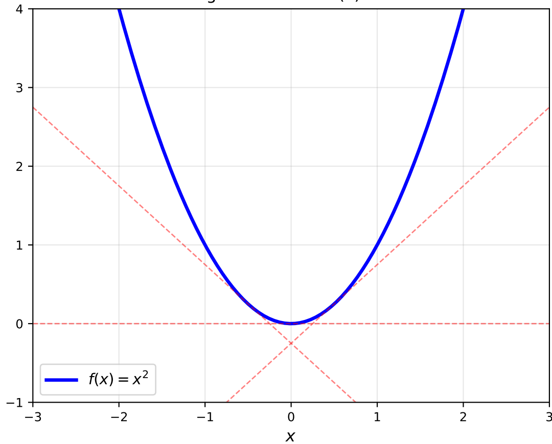
Original Function: f(x) = x^2
