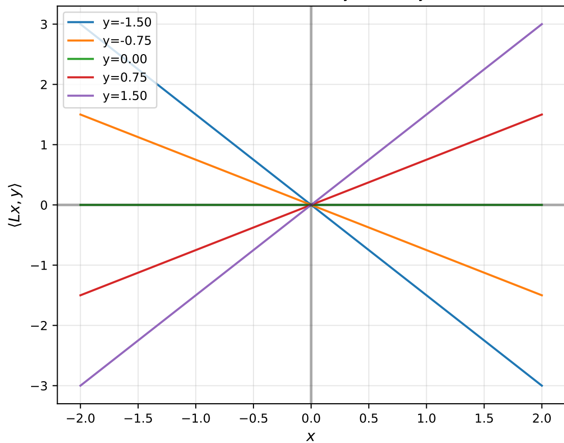
Von Neumann: \min(x) \max(y) = \max(y) \min(x)
