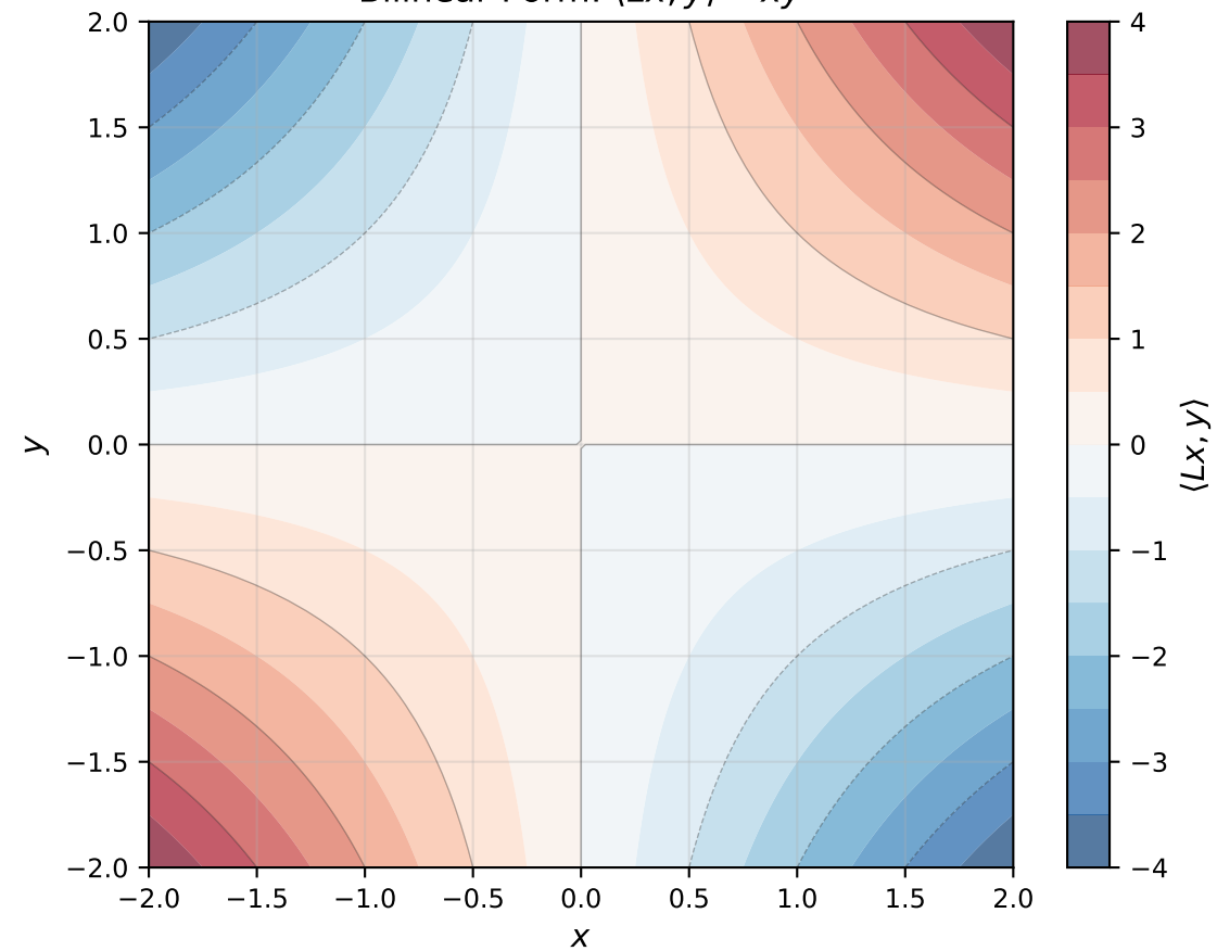
Bilinear Form: \langle Lx, y \rangle = xy
